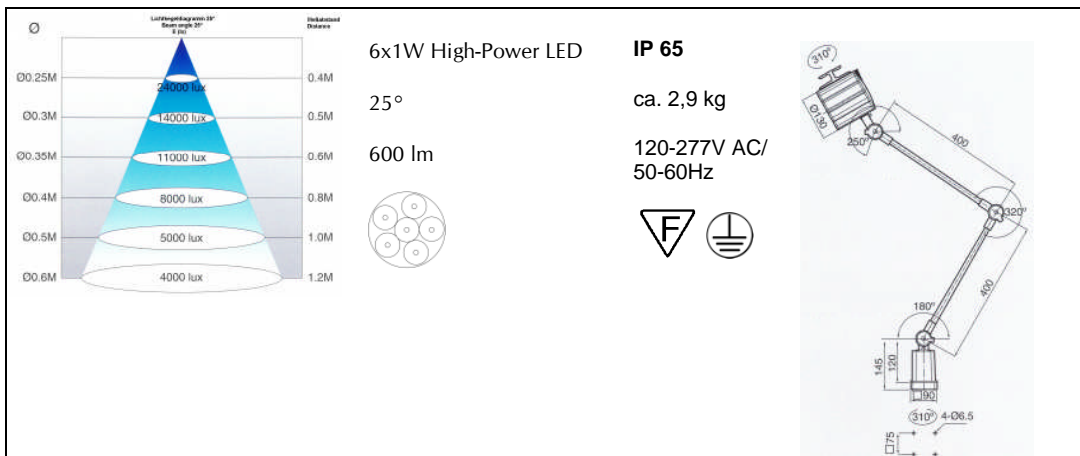
672.95.02-CH / IP 65 / RTL
